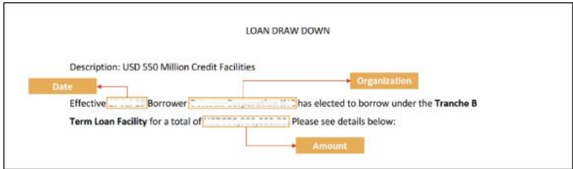
Figure 281: Annotator
