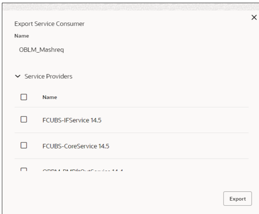
Figure 263: JSON Export
