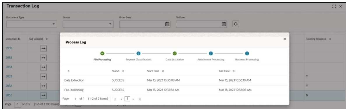
Figure 302: Execution Flow
