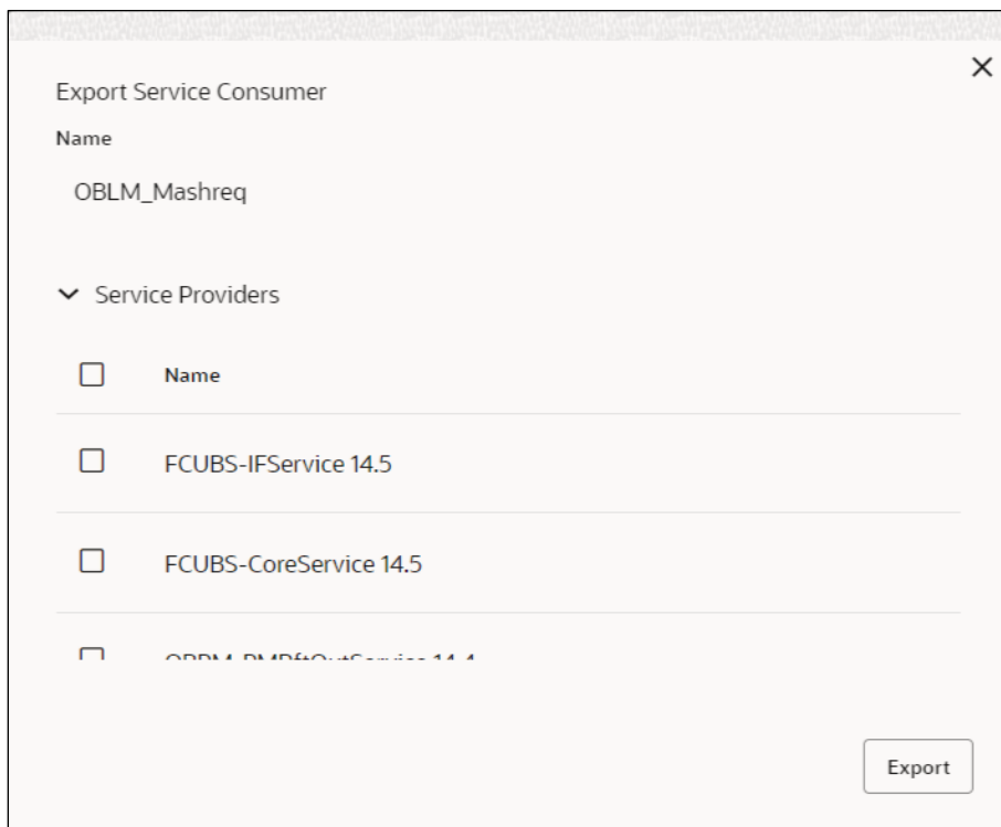
Figure 131: JSON Export
