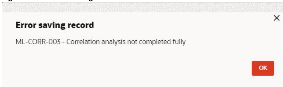
Figure 311: Error Message
