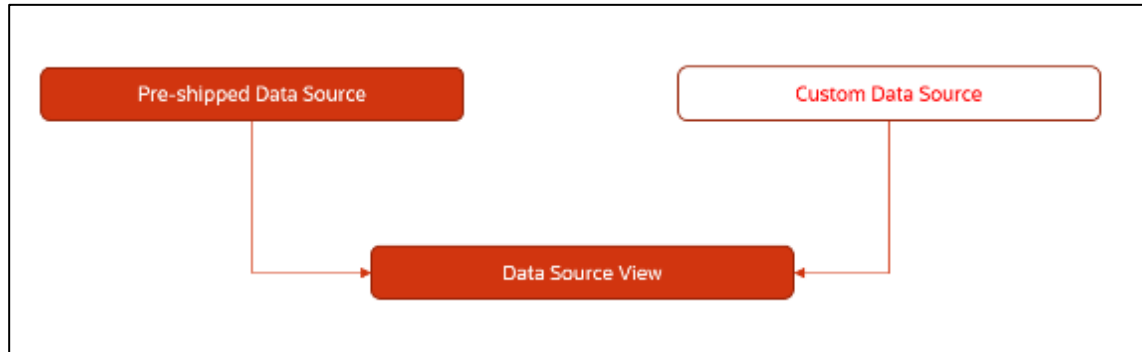
Figure 314: Data Extensibility
