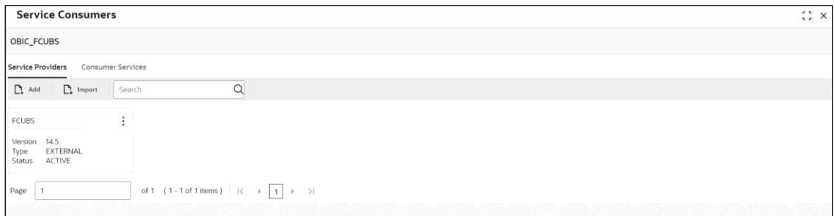
Figure 134: Service Providers
