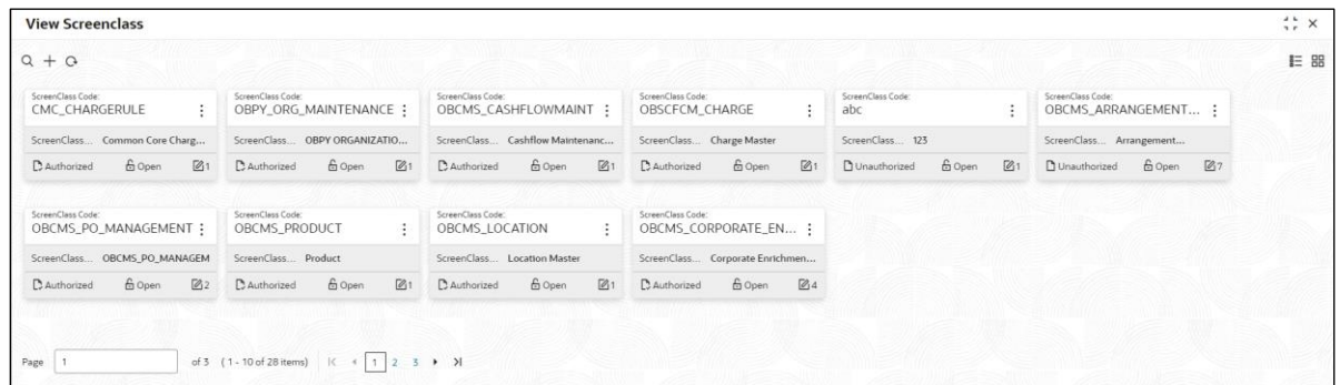
Figure 86: View Screenclass
